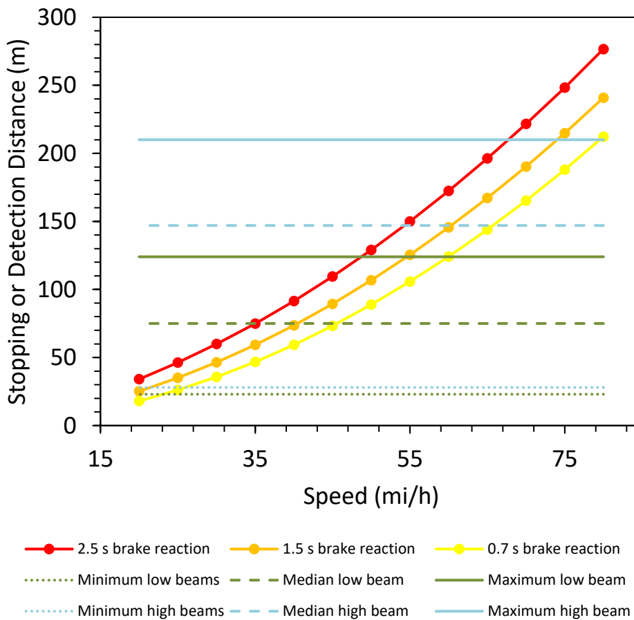
Figure 25. Stopping Distances and Detection Distances for Large Mammals
