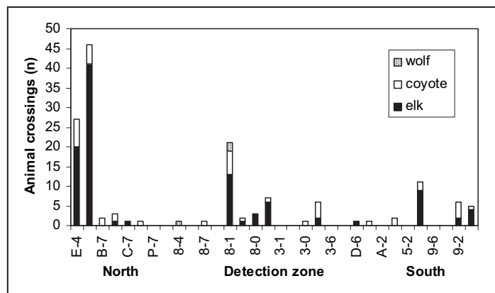
Figure 5. The number of recorded crossings for elk, coyote and wolf through snow tracking between 26 January 2005 and 14 February 2005, 18 February 2005 and 21 February 2005, and 25 February 2005 and 28 February 2005. See figure 1 for the exact location of the detection zones.
